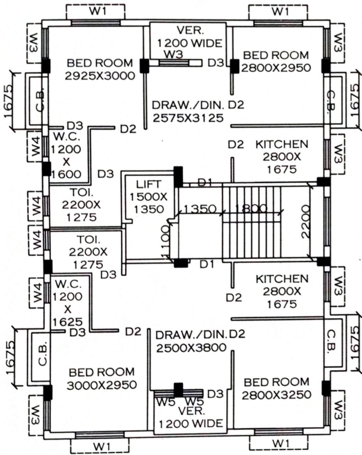
FIRST, SECOND & THIRD FLOOR PLAN
